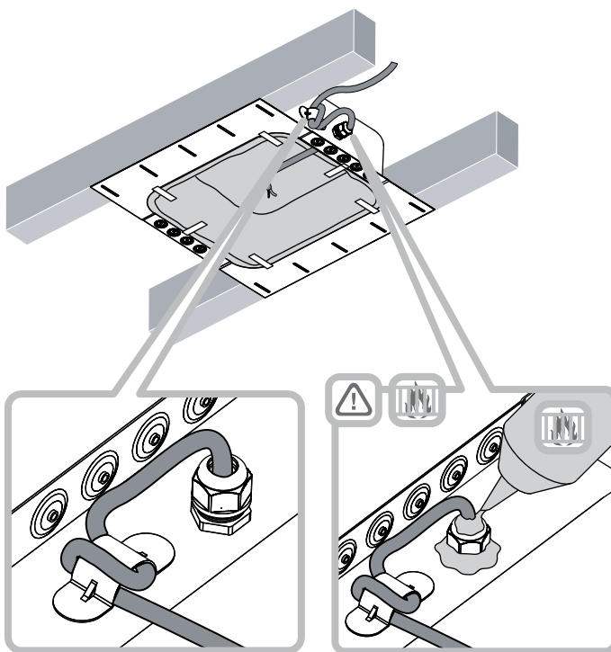
Diagram 10 Back-box stud (joists) installation
